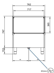
VISTA FRONTEALE FRONTAL VIEW - VUE DE FACE - VISTA FRONTAL
