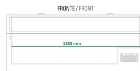
FRONTE / FRONT
