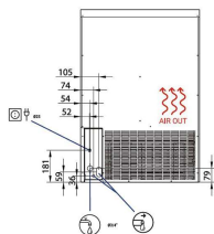
VISTA POSTERIORE REAR VIEW - VUE ARRIÈRE - VISTA TRASERA
