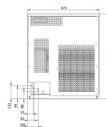
VISTA POSTERIORE REAR VIEW - VUE ARRIÈRE - VISTA TRASERA
